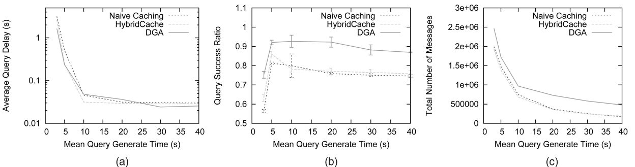
Fig. 6. Varying mean query generate time in spatial data access pattern with v_{max} = 10 \text{ m/s} . (a) Average query delay. (b) Query success ratio. (c) Total number of messages.
