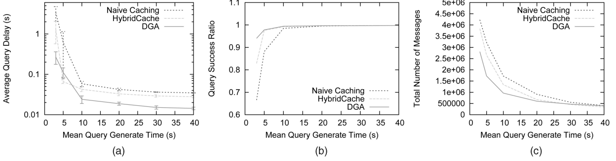
Fig. 4. Varying mean of query generate time on random data access pattern. (a) Average query delay. (b) Query success ratio. (c) Total number of messages.
