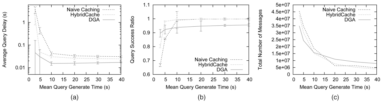
Fig. 11. Varying mean query generate time on spatial data access pattern with cache update in static networks. Here, the data expiry model is TTL-per-request, and the cache update model is cache deletion. (a) Average query delay. (b) Query success ratio. (c) Total number of messages.
