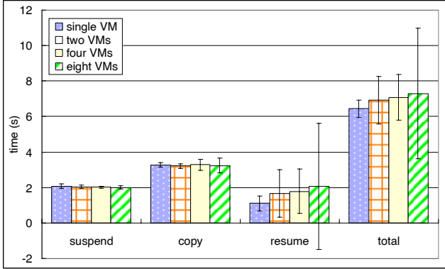
Figure 6: The per-VM migration times when different numbers of VMs, each with a 256MB memory, were migrated in sequence. A local disk on the destination host is used to store the migrated VM state.
