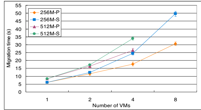
Figure 15: The comparison of total migration times for a sequence of VMs between parallel and sequential migration.
