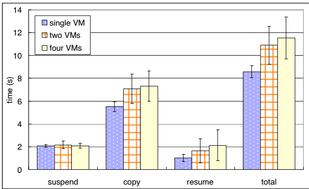
Figure 8: The per-VM migration times when different numbers of VMs, each with a 512MB memory, were migrated in sequence. A local disk on the destination host was used to store the migrated VM state.
