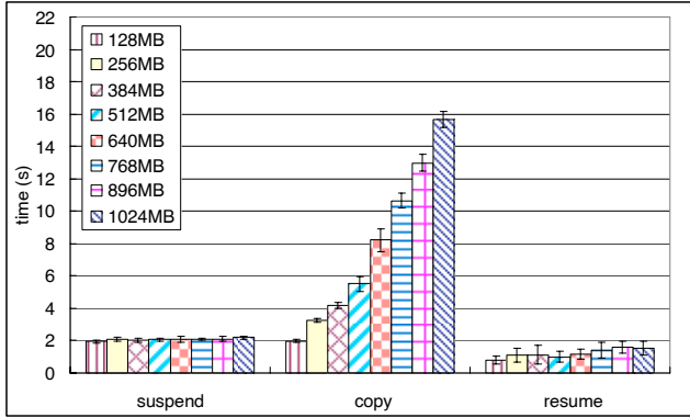
Figure 2: The times needed for the three phases of migrating a single VM with different memory sizes. A local disk on the destination host was used to store the migrated VM states.
