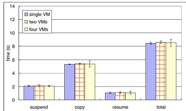
Figure 9: The per-VM migration times when different numbers of VMs, each with a 512MB memory, were migrated in sequence. A RAMFS on the destination host was used to store the migrated VM state.
