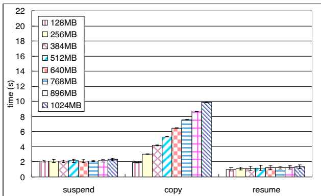
Figure 4: The times needed for the three phases of migrating a single VM with different memory sizes. A RAMFS on the destination host was used to store the migrated VM states.
