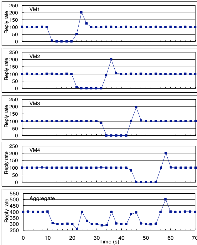
Figure 14: The throughputs of web servers running on four VMs that were under migration.
