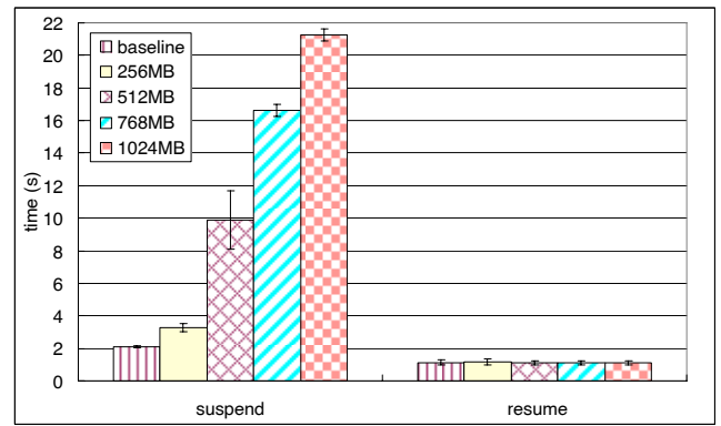
Figure 5: The times needed for the suspend and resume phases of migrating a VM with different amounts of continuously modified memory.
