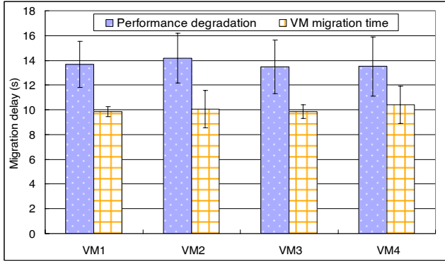
Figure 10: The migration time and performance degradation when four VMs were migrated in sequence, each with 512MB memory and a CPU-intensive benchmark running inside.
