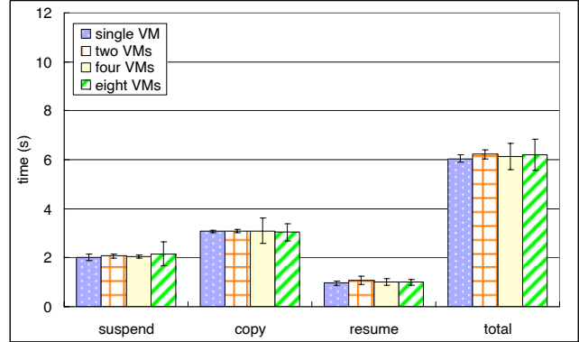
Figure 7: The per-VM migration times when different numbers of VMs, each with a 256MB memory, were migrated in sequence. A RAMFS on the destination host was used to store the migrated VM state.
