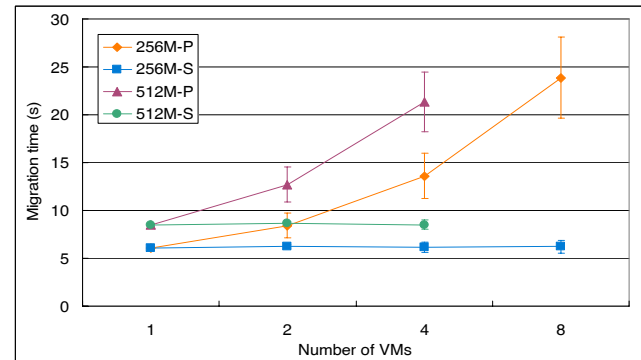
Figure 16: The comparison of per-VM migration times for a sequence of VMs between parallel and sequential migration.
