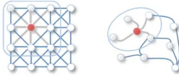
Left: Convolution on a regular graph such as an image. Right: Convolution on the arbitrary graph structure. Figure from " A Comprehensive Survey on Graph Neural Networks "
